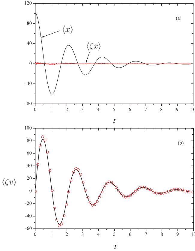
FIG. 1. (Color online) Results from numerical stochastic simulations to verify Eqs. (4.15) and (4.16). (a) \langle x \rangle and \langle \zeta x \rangle versus time. (b) Left-hand side (circles) and right-hand side (solid line) of Eq. (4.15). We have performed averages over 10^6 realizations, \delta t = 0.005 , w_0 = 0.2 , \omega = 3 , b = 1 , and \beta = 5 .
