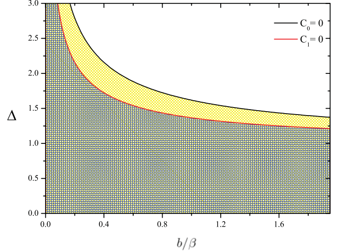
FIG. 3. (Color online) Stability diagram in the \Delta - b/\beta plane for the damped oscillator under white shot noise for \omega/\beta = 0.1 . We represent the critical curves provided by the conditions C_0 = 0 and C_1 = 0 . In the upper (white) region, the oscillator is unstable in the mean and in the mean square, \langle x \rangle \rightarrow \infty and \langle x^2 \rangle \rightarrow \infty as t \rightarrow \infty . In the intermediate (yellow) region, it is stable in the mean but unstable in the mean square, \langle x \rangle \rightarrow 0 and \langle x^2 \rangle \rightarrow \infty as t \rightarrow \infty . In the lower (blue) region, it is stable both in the mean and in the mean square, \langle x \rangle \rightarrow 0 and \langle x^2 \rangle \rightarrow 0 as t \rightarrow \infty .
