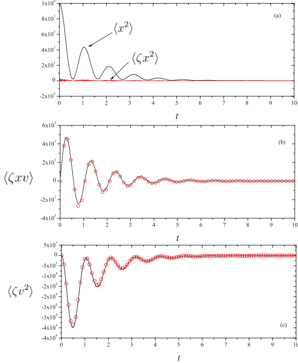
FIG. 2. (Color online) Results from numerical stochastic simulations to verify Eqs. (4.29), (4.30), and (4.31). (a) \langle x^2 \rangle and \langle \zeta x^2 \rangle versus time. (b) Left-hand side (circles) and right-hand side (solid line) of Eq. (4.30). (c) Left-hand side (circles) and right-hand side (solid line) of Eq. (4.29). We have performed averages over 10^6 realizations, \delta t = 0.005 , w_0 = 0.2 , \omega = 3 , b = 1 , and \beta = 5 .
